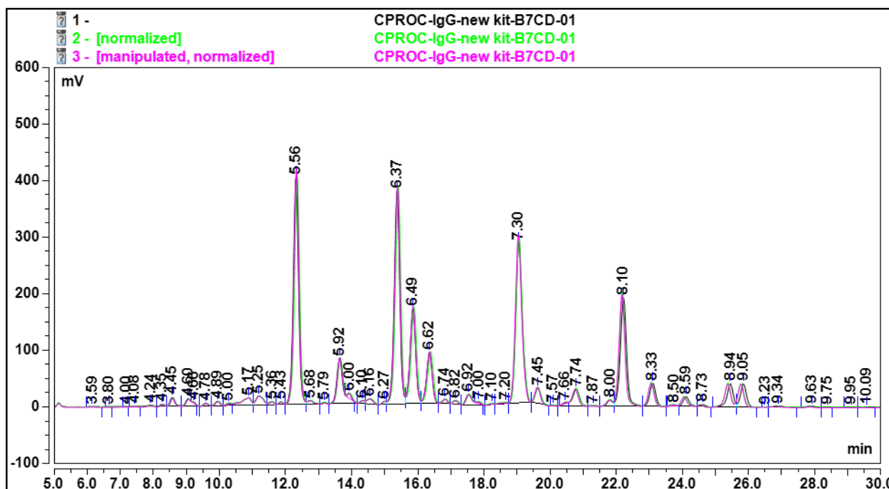
Figure 1: BEH Glycan column UHPLC profile of procainamide labeled N-glycans released from human IgG by PNGase F digestion
