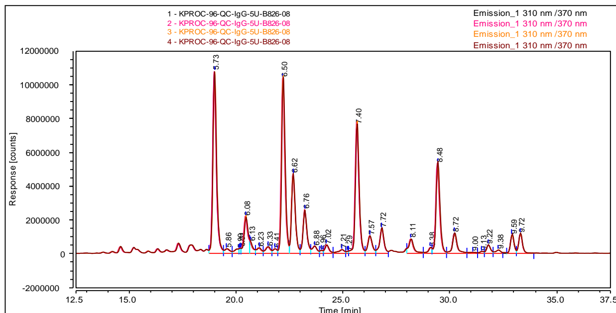
Figure 1: BEH Glycan column UHPLC profile of procainamide labeled N-glycans released from human IgG by PNGase F digestion
