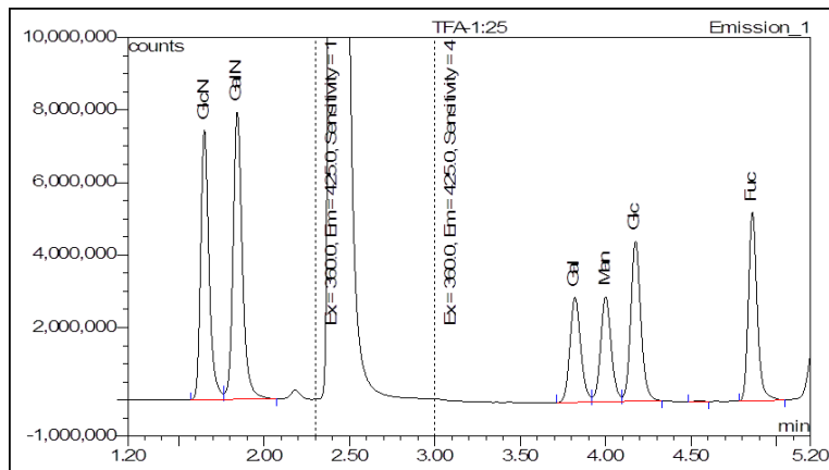
Figure 1. LudgerSep-uR2 profile of CM-Mono-Mix-10 -2AA labelled - monosaccharide gradient. Date of Analysis – 29 April 2013.
