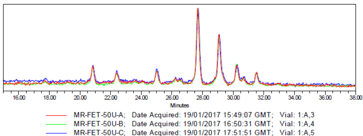
Figure 1: HILIC-UHPLC profile overlay of 3 x 2AB labelled GCP-FET-50U (B719-04) released using LL-MR-A2
