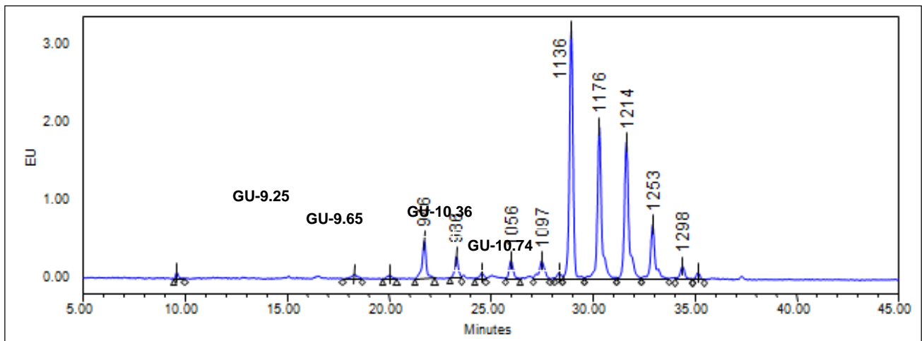
Figure 1: HILIC HPLC profile of 2-AB labelled Fetuin N-glycans, released by PNGase F from GCP-FET-50U batch B427-01 run on Waters BEH Glycan column.
