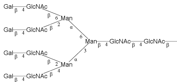
Text Notation
