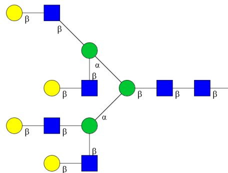
CFG Notation
