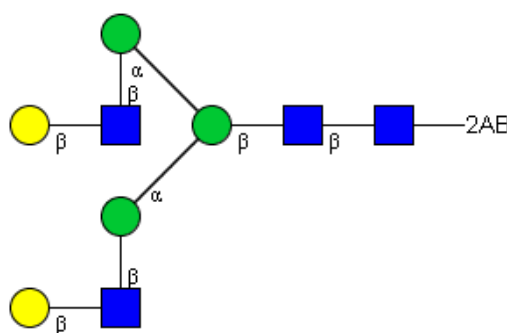
CFG Notation
