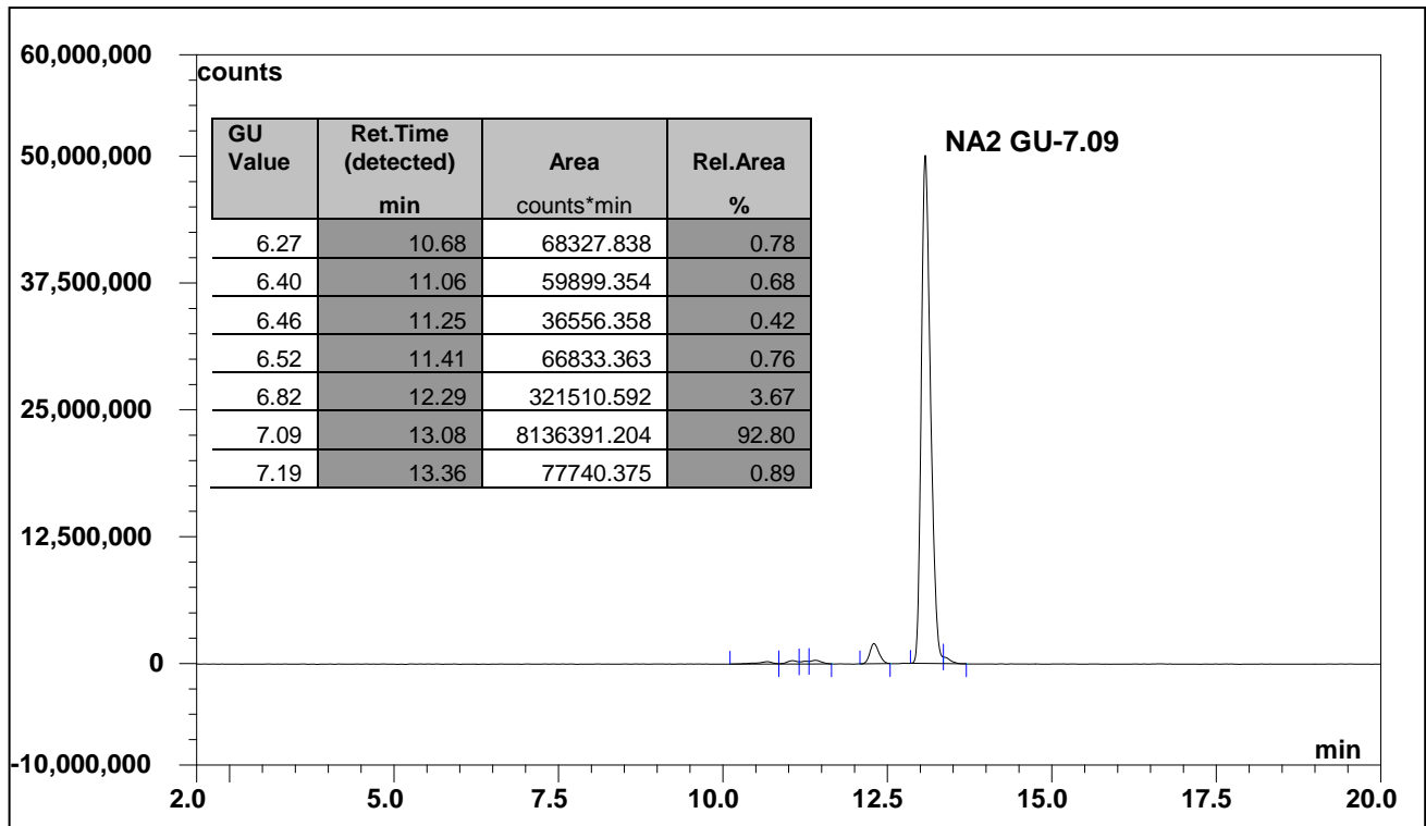
Figure 1: HILIC HPLC profile of 2AB labelled NA2 glycan (see method conditions below) (Cat. #: CAB-NA2-01, Batch B335-02).
