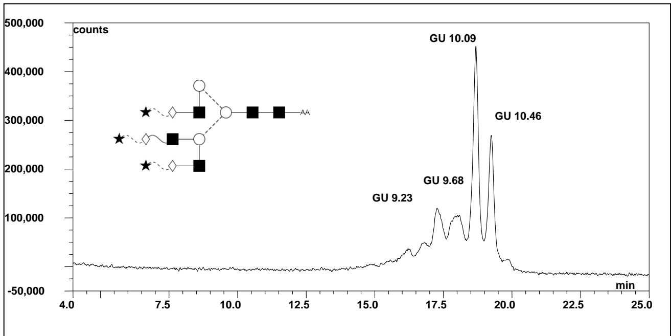
Figure 1: LudgerSepN2 HPLC profile of 2AA labeled A3 glycan (Cat. #: CAA-A3-01, Batch B1AL-02).
